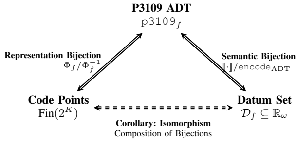
Fig. 1: The three-way isomorphism between code points, the algebraic ADT, and the datum set.
