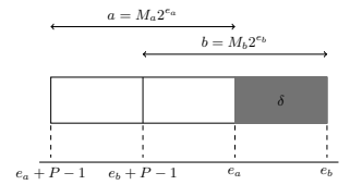
(b) Visualization of \delta = a + b - s
