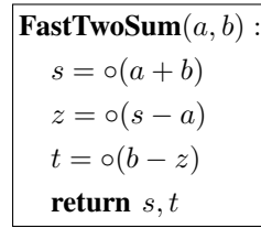
(a) Original FastTwoSum algorithm
