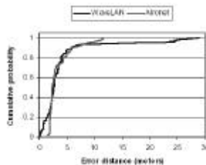
Fig: CDF of the Error Distance
