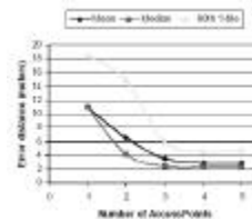
Fig: Impact of the number of APs on the error distance.
