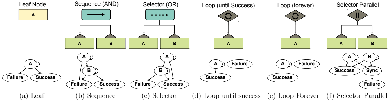
Figure 4: Control flow graphs for the different control nodes used in Behavior Trees.
