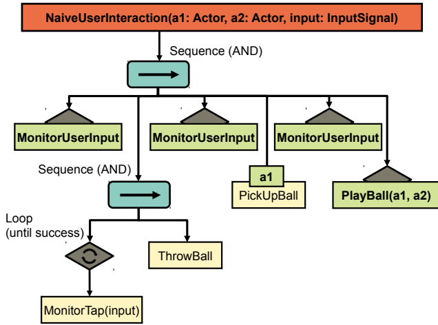
Figure 2: Handling user interaction in a traditional Behavior Tree. The MonitorUserInput subtree is required at all points in the narrative tree where the user selects how the narrative proceeds, resulting in unnecessary large trees.
