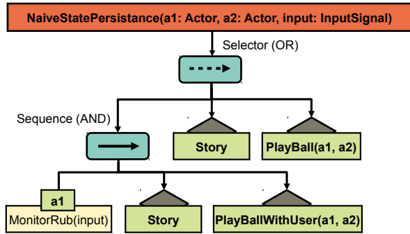
Figure 3: A naive approach to handle state persistence in Behavior Trees.
