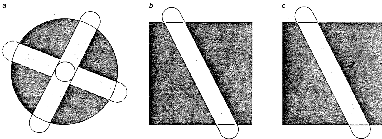
RECEPTIVE FIELDS of various cells in the visual pathway are compared. Retinal ganglion cells and neurons in the lateral geniculate nucleus have circular fields with either an excitatory center and an inhibitory surround ( a ) or the opposite arrangement. A spot of light falling on the center stimulates a response from such a cell; so does a bar of light falling on the field in any orientation, provided it falls on the center. In the visual cortex there is a hierarchy of neurons with in-
