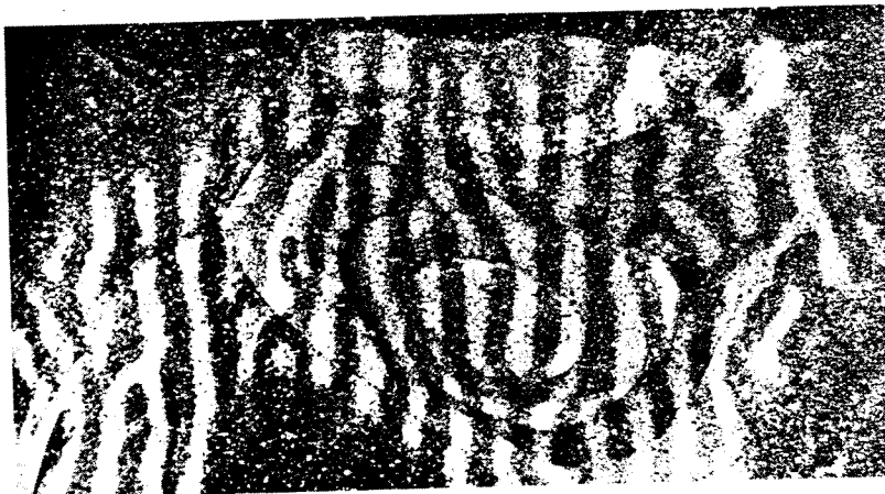
ANATOMICAL CONFIRMATION of ocular-dominance columns came from various staining methods and from axonal-transport autoradiographs such as those shown in color on page 85. This composite autoradiograph visualizing the pattern over an area some 10 millimeters wide was made by cutting out and pasting together the regions representing layer IV in a number of parallel sections; the one in bottom illustration on page 85 and others at different depths.
