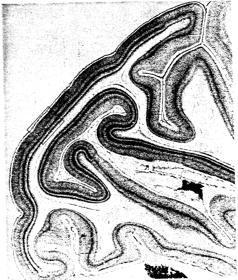
SECTION OF VISUAL CORTEX along the colored line in the illustration on the opposite page was stained by the Nissl method, which makes cell bodies but not fibers visible. The visual cortex is seen to be a continuous layered sheet of neurons about two millimeters thick. The black rectangle outlines a section like the one that is further enlarged in the illustration below.
