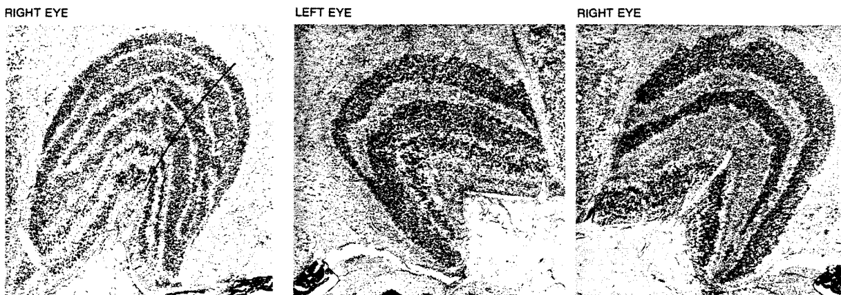
LATERAL GENICULATE NUCLEUS of a normal monkey ( left ) is a layered structure in which cells in layers 1, 4 and 6 (numbered from bottom to top) receive their input from the eye on the opposite side and those in layers 2, 3 and 5 receive information from the eye on the same side. The maps are in register, so that the neurons along
