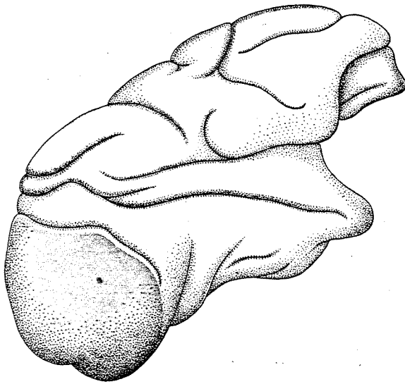
PRIMARY VISUAL CORTX , also known as the striate cortex or area 17, is a region of the cerebral cortex: a layered plate of neurons that envelops the primate brain. In the macaque brain, seen here from the side ( left ) and from above and behind ( right ), the primary visual cortex ( colored areas ) occupies most of the exposed surface of
