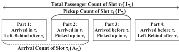
Fig 12: Inferring Previous Arrival Count \mathbb{A}_{\tau_i}
