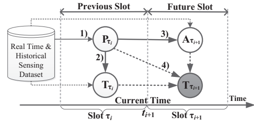
Fig 9: Dmodel Inference Overview
