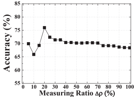
Fig 17: \Delta\rho vs. Accuracy
