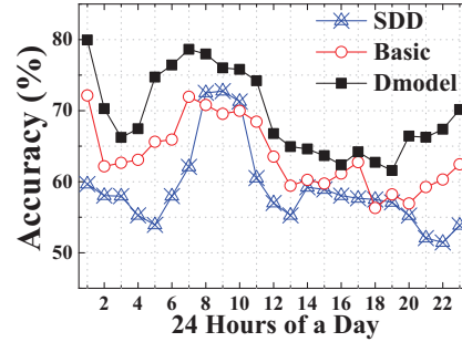
Fig 15: Hourly Average Accuracy
