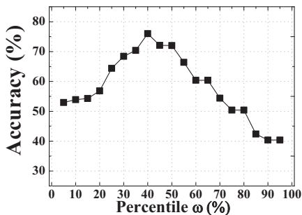
Fig 18: \omega vs. Accuracy
