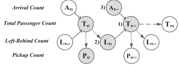
Fig 8: Passenger Demand in a Hidden Markov Model
