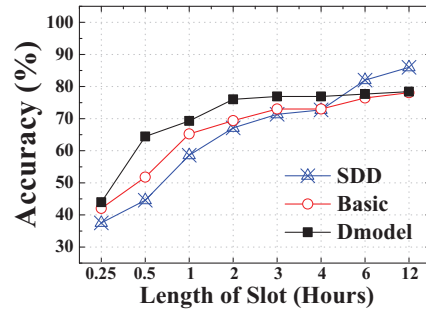
Fig 16: Effects of Slot Lengths
